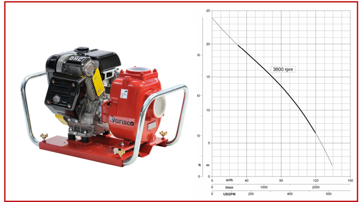
3" J 4-100
