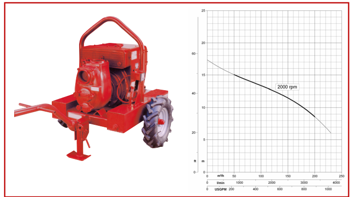
4" J 5-180
