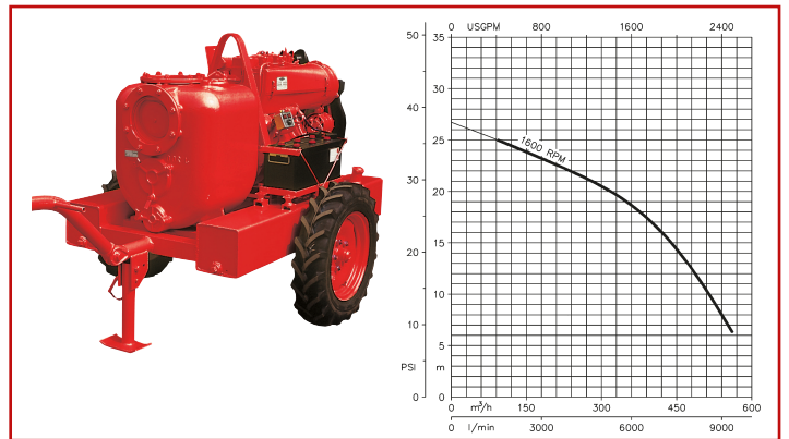
6" J 8-300
